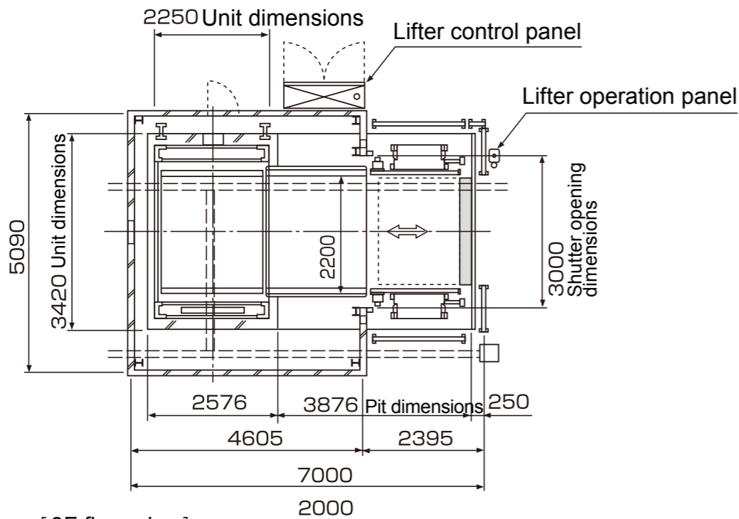
[ 3F floor plan ]
