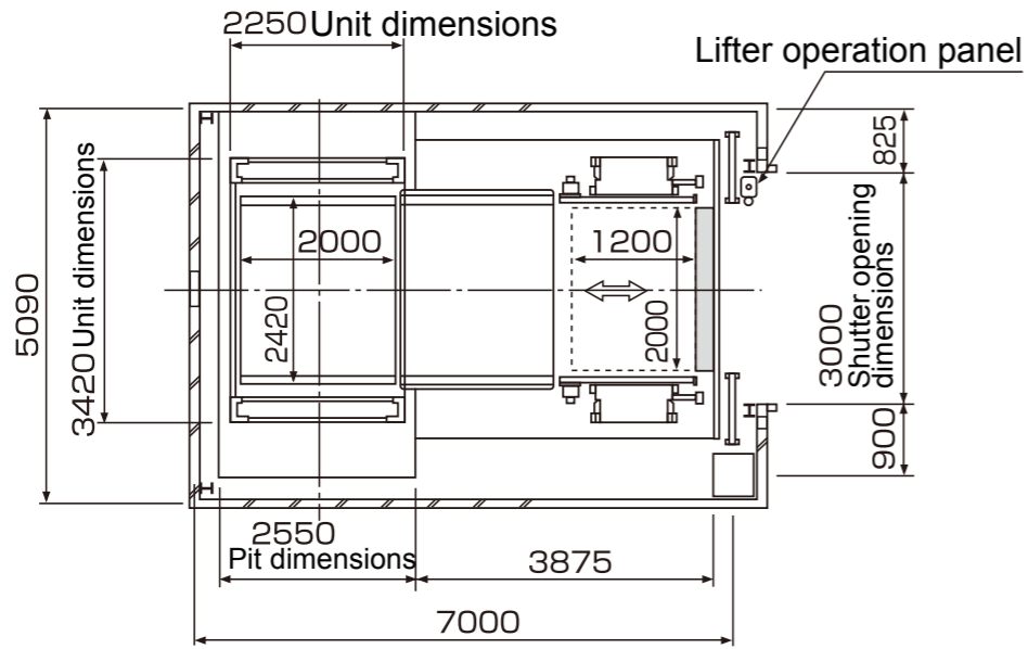
[ 1F floor plan ]
