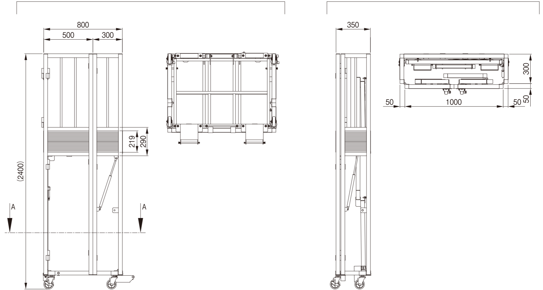
Folded state
